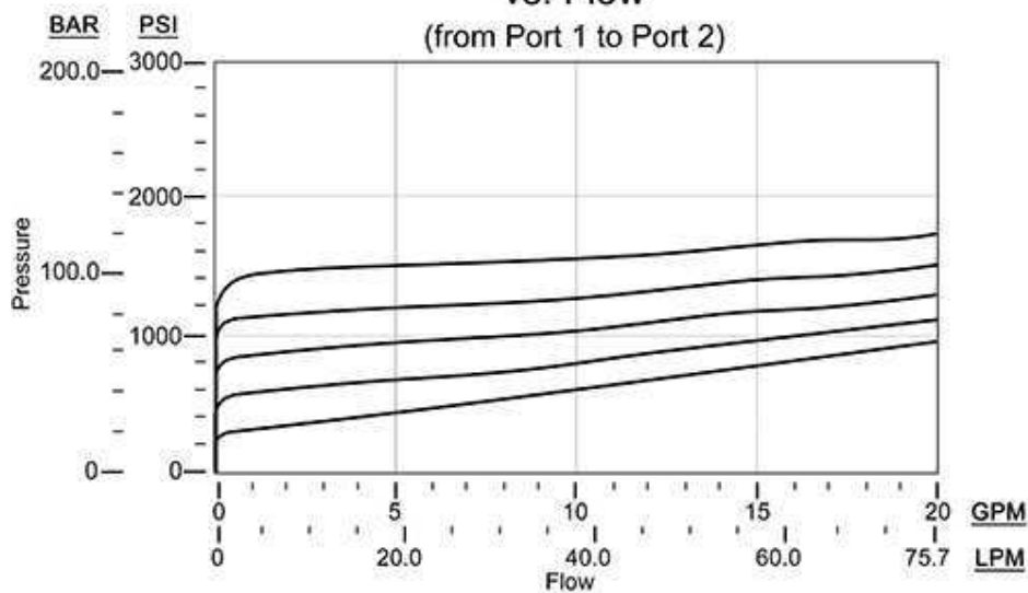
RBUY - *A* Typical Pressure Differential vs. Flow (from Port 2 to Port 1)
