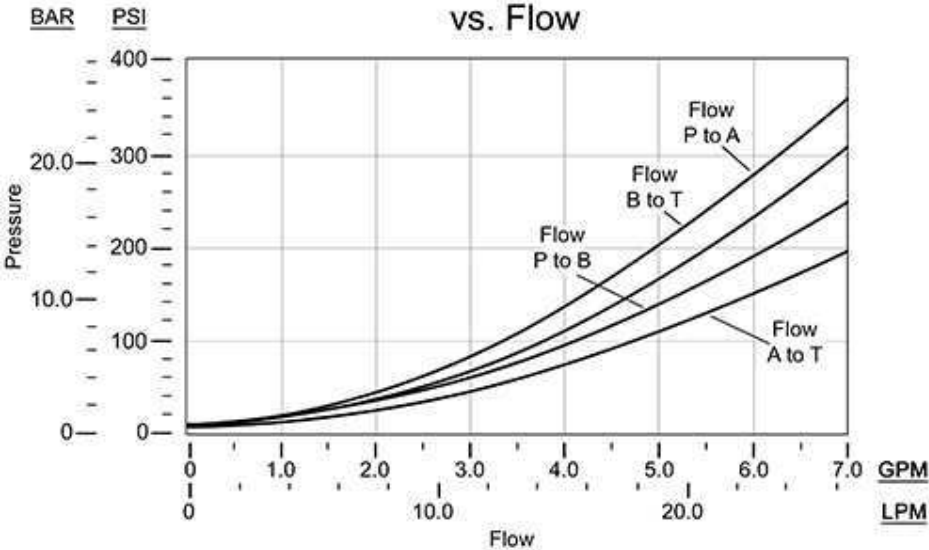
DNUC-XHN Pressure Differential vs. Flow
