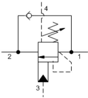
4-Port Vented
