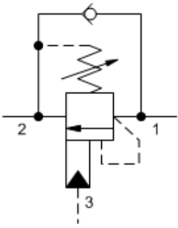
3-Port Non-vented
