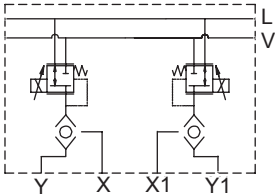
SCHEME 0
