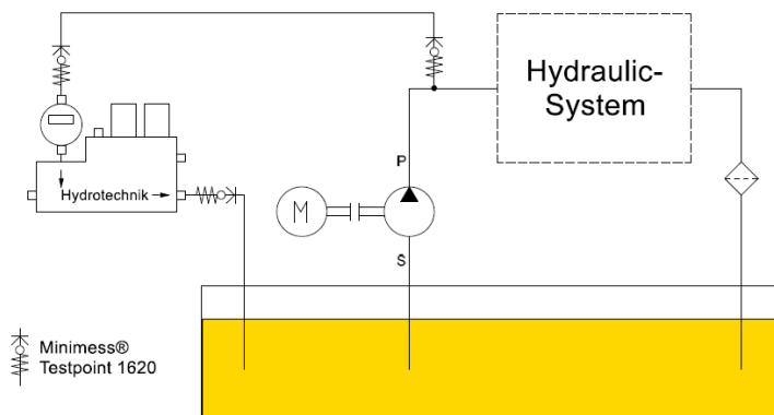
Figure 5: Installation situation of the CX 197; left: recommended installation; right: alternative installation
