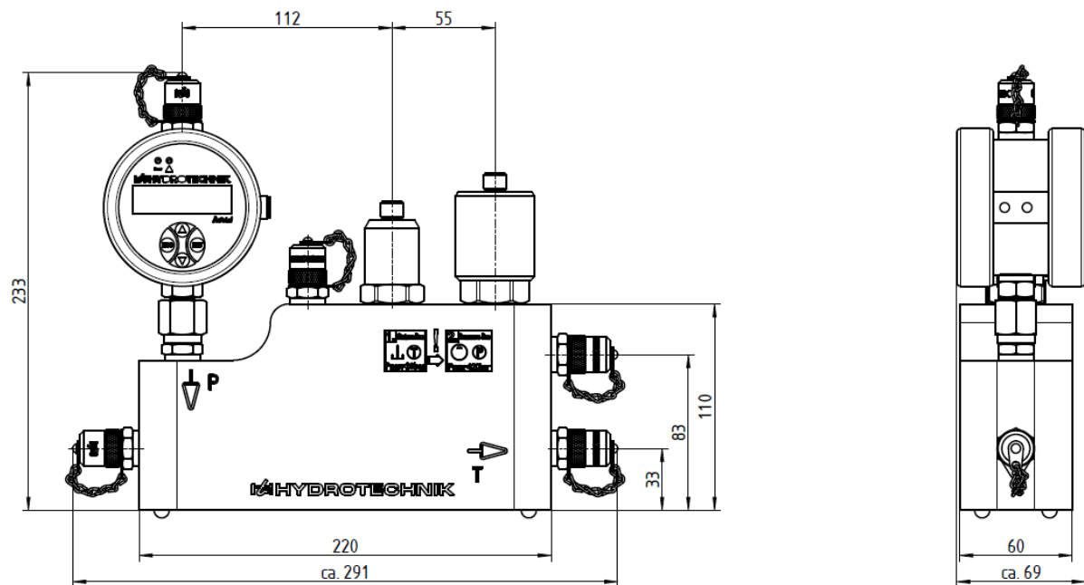
Figure 1: Technical drawing CX 197
