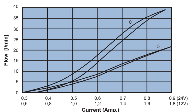
Graph flow/current with \Delta p from 2 to 1
